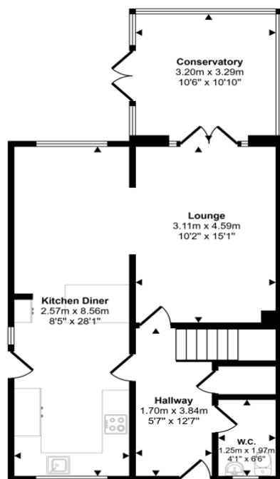
Ground Floor Approx 61 sq m / 659 sq ft
