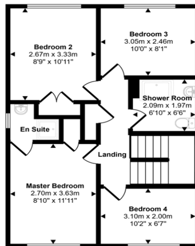
First Floor Approx 51 sq m / 549 sq ft
