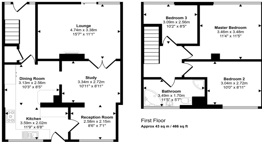
Ground Floor Approx 56 sq m / 604 sq ft
